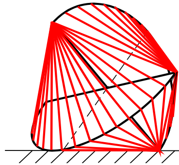
Fig. 3: By connecting all corresponding bearing-surface points of the wobbler to each other the so-called connecting developable are obtained.
